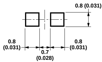
Figure 11. Recommended soldering pattern for HSMW-C191 and HSMW-C190.
